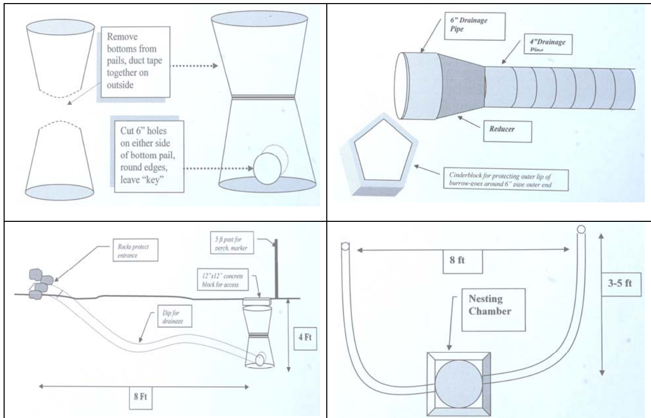
Figure 7. Design drawings for the burrow system being used by the Wildlife Resources Institute (California).
