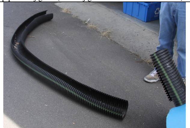
Figure 22. 10-foot tunnel section of 6-in. flexible drain line. A 3 in. wide “walkway” has been cut out. This will be placed face-down, so the owls can walk on natural dirt. A jigsaw is used to cut the walkway out of the flex pipe.
