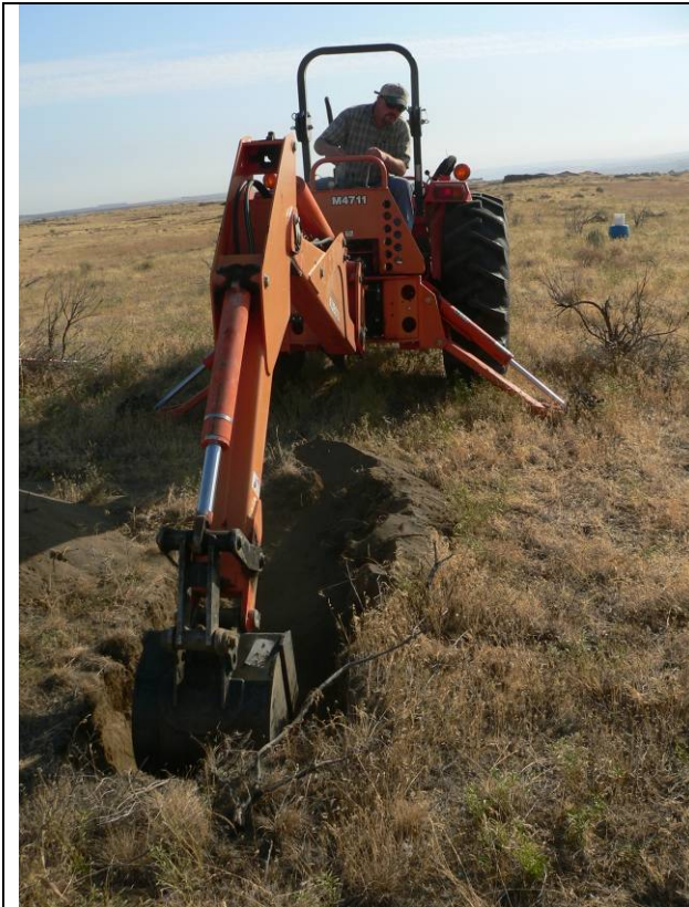
Backhoe digging main hole for burrow chamber; the bottom of the burrow chamber will be 36 in.es below ground level.
