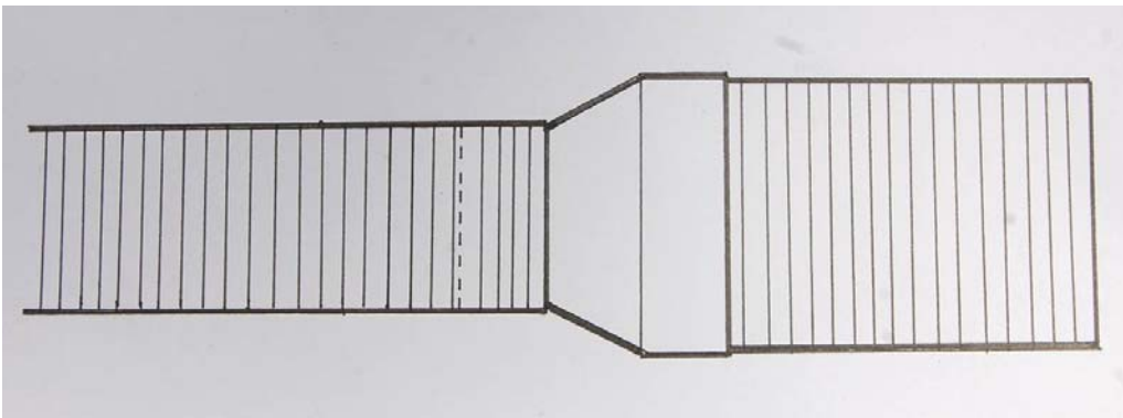
Figure 35. Anti-predator patio for 10 cm (4 in.) tunnel. Drawing of completed anti-predator patio unit with the 3 components: 4 in. main tunnel, a 4-6 in. connector, and a 6 in. diam. x 12 in. long patio section. About 1 in. of dirt is placed inside the patio unit (and a lesser amount in the tunnel) to level the walkway for the owls. Entrance is from the right.
