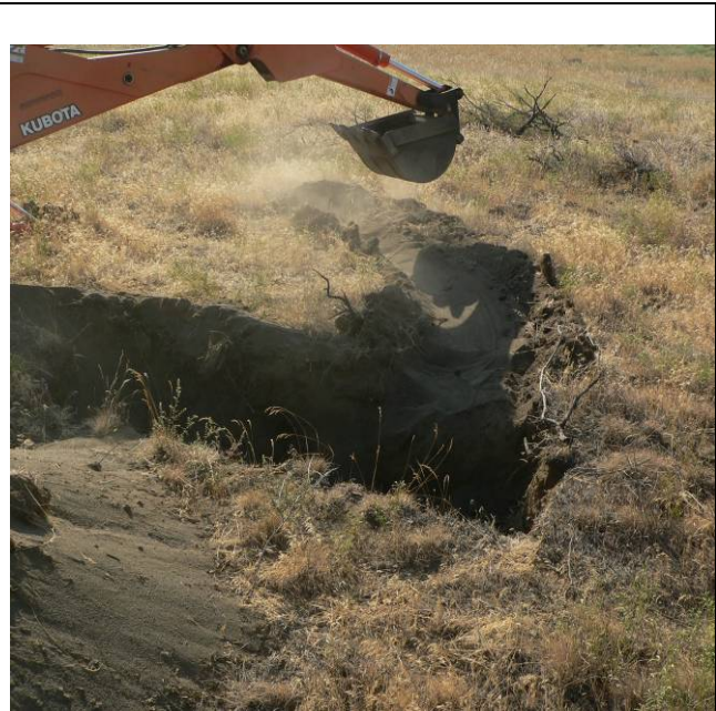
Trench for the burrow tunnel is done with a sweeping motion of the backhoe bucket. In this image it is a left-swinging and upward motion. This gives the trench an appropriate arc for the main tunnel. Some hand digging may be necessary (to get the trench deep enough) right where the main tunnel meets the collar/burrow chamber.
