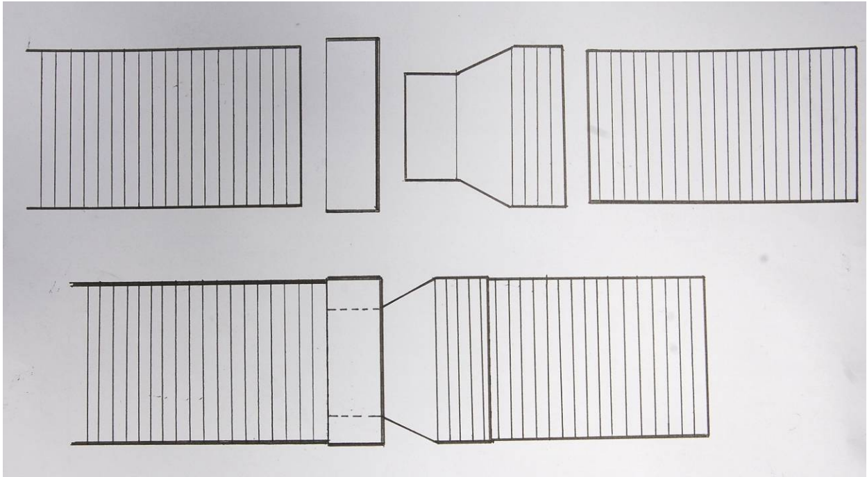
Figure 34. Anti-predator patio for 15 cm(6 in.) tunnel. Top drawing shows the four components for the anti-predator patio (L to R): 6 in. dia. main tunnel, a 6 in. cap (with 4 in. dia. hole cut out of it), a 4-to-6 in. connector, and a 6 in. dia. x 12 in. patio section. Liquid Nails (or similar adhesive) is used to connect the cap, connector, and patio section together so they become a solid unit. Bottom image shows the completed patio unit. Entrance is from the right. About 1 in. of dirt is placed inside the patio unit and tunnel to level the walkway for the owls. The exact dimensions of these components may vary based on the materials available in your location.
